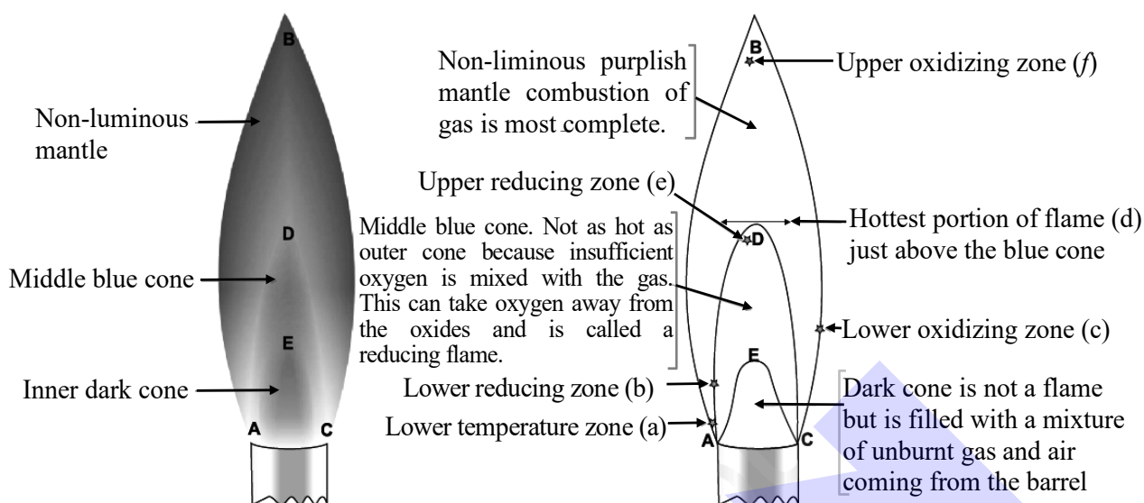
Fig.1.13 : Zones of flame of Bunsen burner
