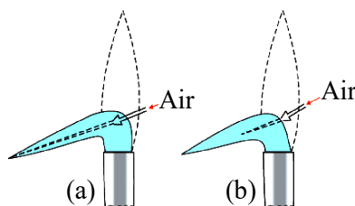
Fig.1.7 : Obtaining oxidizing and reducing flame (a) oxidizing flame; and (b) Reducing flame
